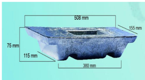
Figure 12: Lead casting
