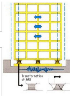
Figure 3: Deformation of structures with insulation
