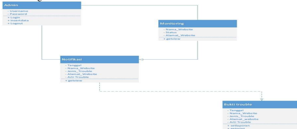
Gambar 3.2. Class Diagram
