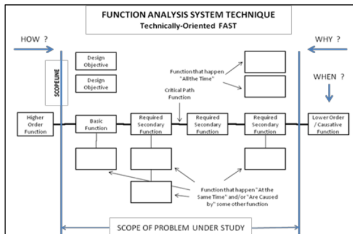
Gambar II.3 Diagram FAST
