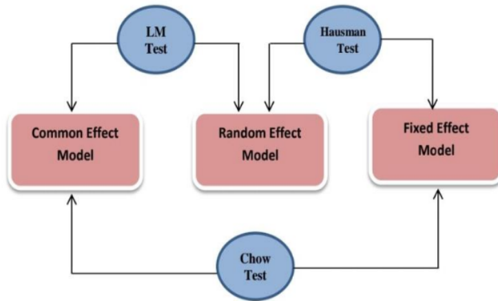
Figure 2: Model Fit Test
