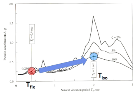
Fig. 13: Comparison of fixed-base and isolated-base design from spectrum perspective.
