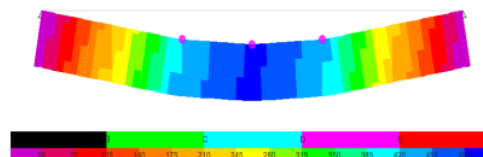
Fig. 10: Stress contour from numerical analysis.
