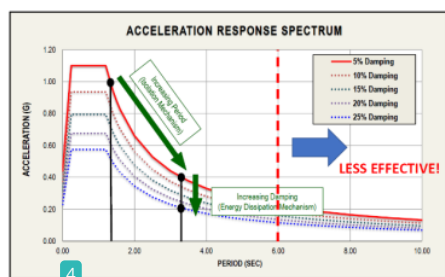
Fig. 14: Comparison of fixed-base and isolated-base design from spectrum perspective.
