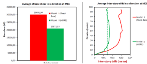
Fig. 20: Base shear and inter-story drift at MCE.
