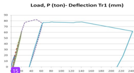
Fig. 9: Load-deflection curve of beam test module.
