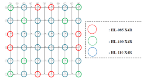
Fig. 19: Layout of HDRB for example building.
