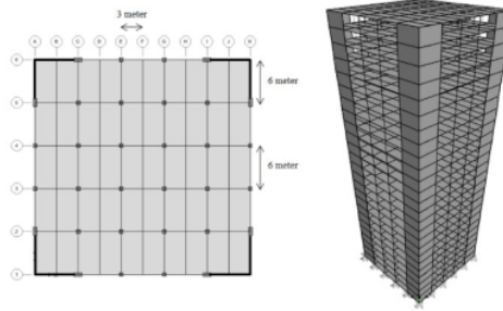
Fig. 18: Example building for study base isolation.
