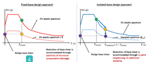
Fig. 12: Comparison of fixed-base and isolated-base design from spectrum perspective.
